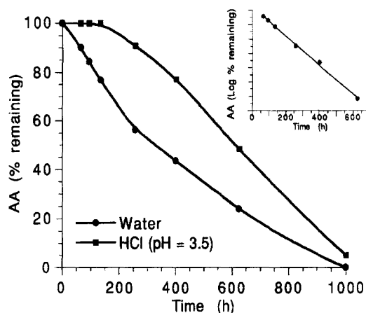
Fig. 1. Degradation with time (h) of L-ascorbic acid (AA) in distilled water and in a pH 3.5 HCl solution. The initial concentration of AA was 3 \times 10^{-4} M and the temperature was kept at 5 \pm 1^\circ\text{C} throughout the experiment. Inset: semilogarithmic plot of AA degradation in distilled water.
